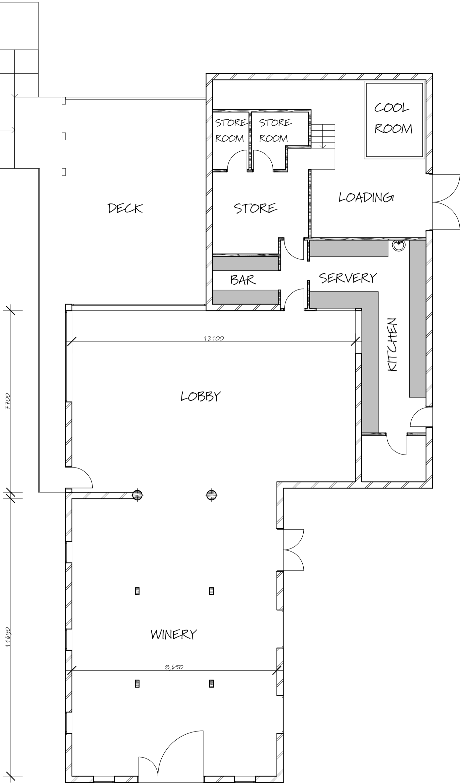
WINERY FLOORPLAN SCALE 1:100 (NOMINAL DIMENSIONS ONLY)
